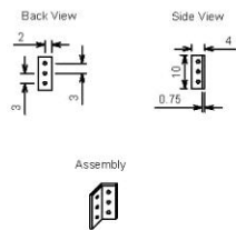
Angle Connection (x4)
